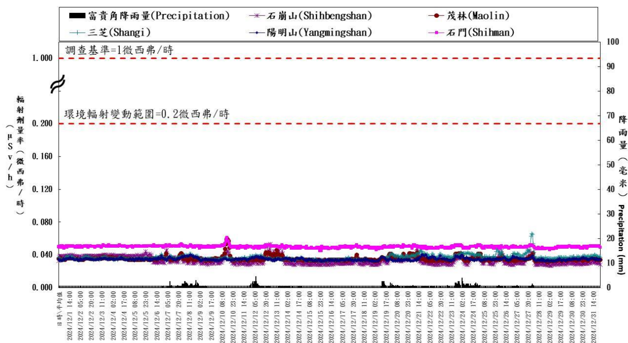
核一廠輻安預警自動監測時平均劑量率(中華民國一百一十三年十二月) Hourly average dose rates around NPP1 in Taiwan (December, 2024)
