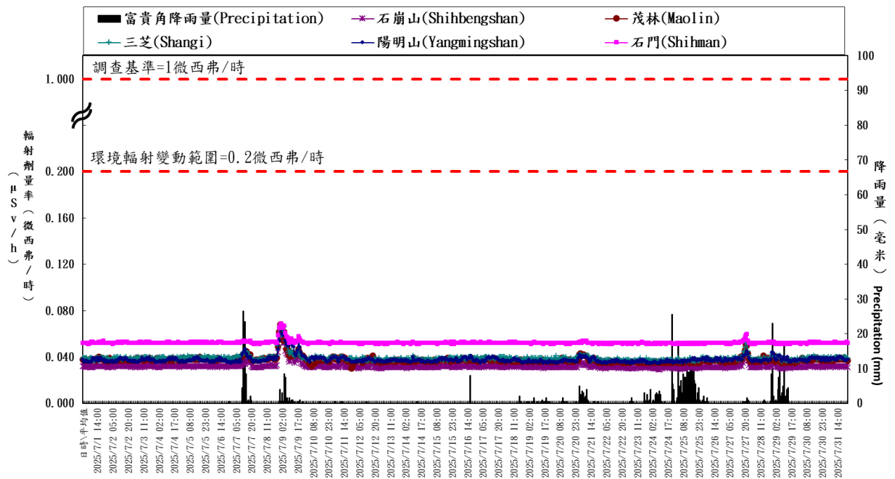
核一廠輻安預警自動監測時平均劑量率(中華民國一百一十四年七月) Hourly average dose rates around NPP1 in Taiwan (July, 2025)
