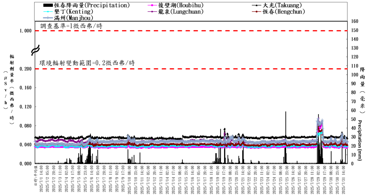
核三廠輻安預警自動監測時平均劑量率(中華民國一百一十四年七月) Hourly average dose rates around NPP3 in Taiwan (July, 2025)
