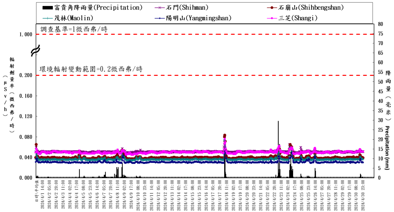
核一廠輻安預警自動監測時平均劑量率(中華民國一百一十三年四月) Hourly average dose rates around NPP1 in Taiwan (April, 2024)
