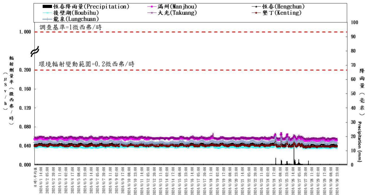
核三廠輻安預警自動監測時平均劑量率(中華民國一百一十三年四月) Hourly average dose rates around NPP3 in Taiwan (April, 2024)
