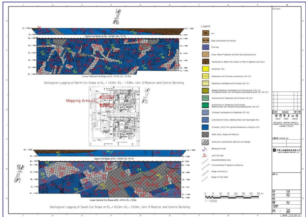
Geological logging of northern and southern cut slope, Unit No. 2 Reactor and Control Building
