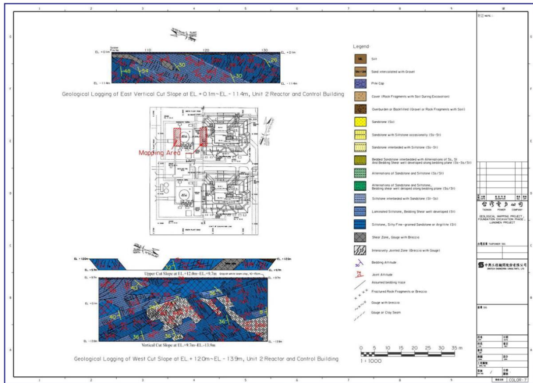
Geological logging of eastern and western cut slope, Unit No. 2 Reactor and Control Building
