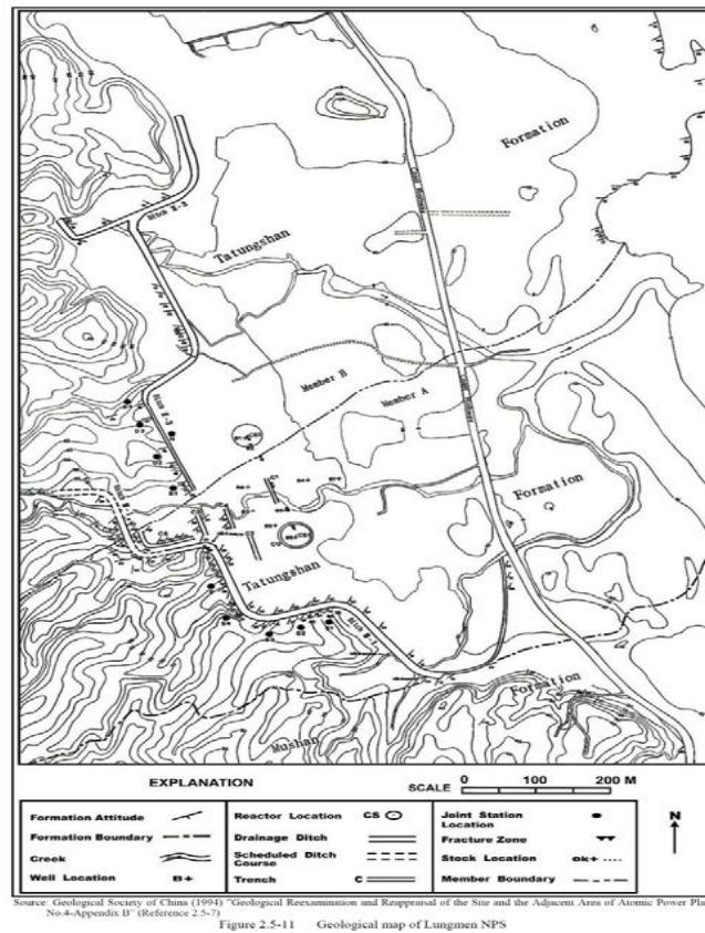
Figure 2.5-11 Geological map of Lungmen NPS
