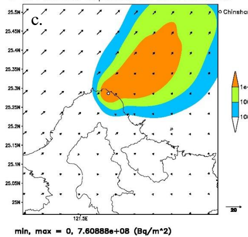
I-131 Surface Deposition on 00Z31MAY2018
