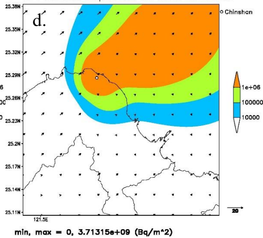
I-131 Surface Deposition on 00Z31MAY2018
