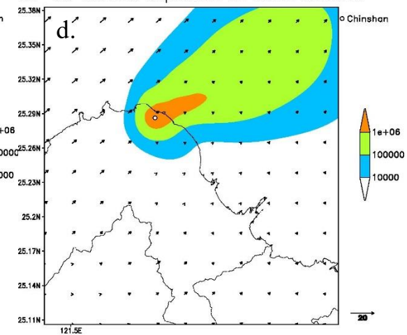
Cs-137 Surface Deposition on 00Z31MAY2018
