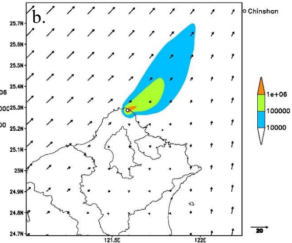
Cs-137 Surface Deposition on 00Z31MAY2018
