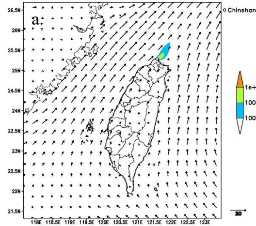
Cs-137 Surface Deposition on 00Z31MAY2018
