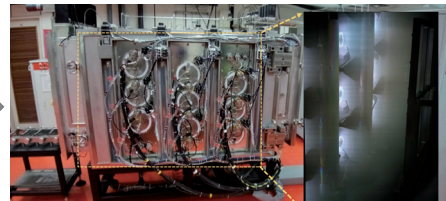
生產與環境永續：低碳環保、低成本電致變色量產機台 Production and environmental sustainability: Low-carbon, environmentally friendly, and cost-effective mass production equipment for electrochromic devices.
